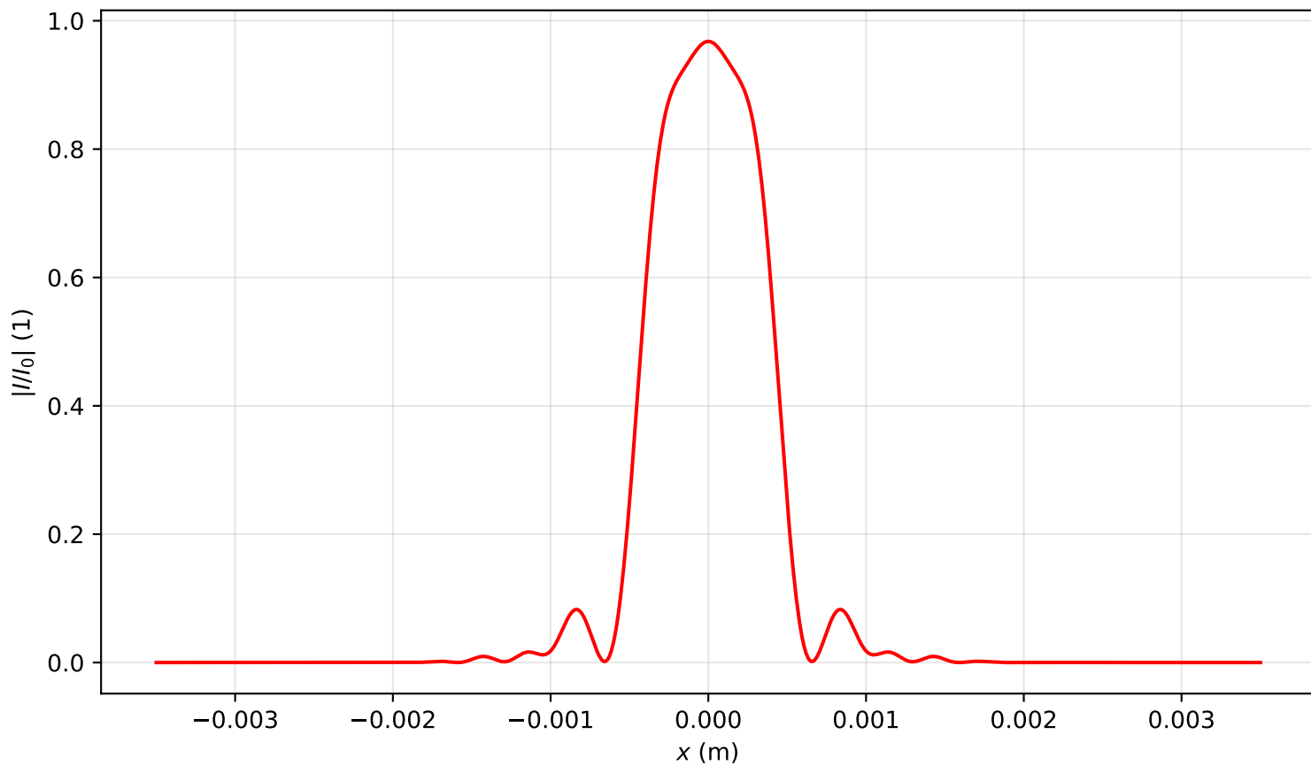
Intensity profile I(x, y = 0, z = 1.672)/I_0 , \text{Pin}=2.0\text{Pcr} , artificial time
